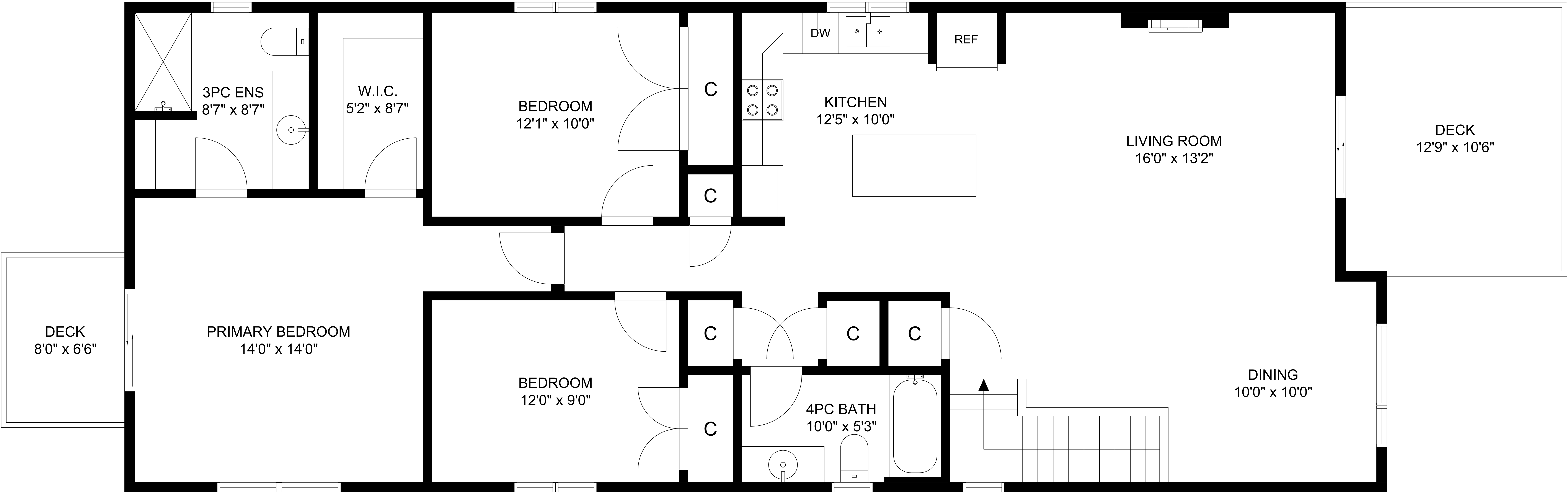
MAIN LEVEL - 1426 SQFT CEILING HEIGHT - 8'0"
