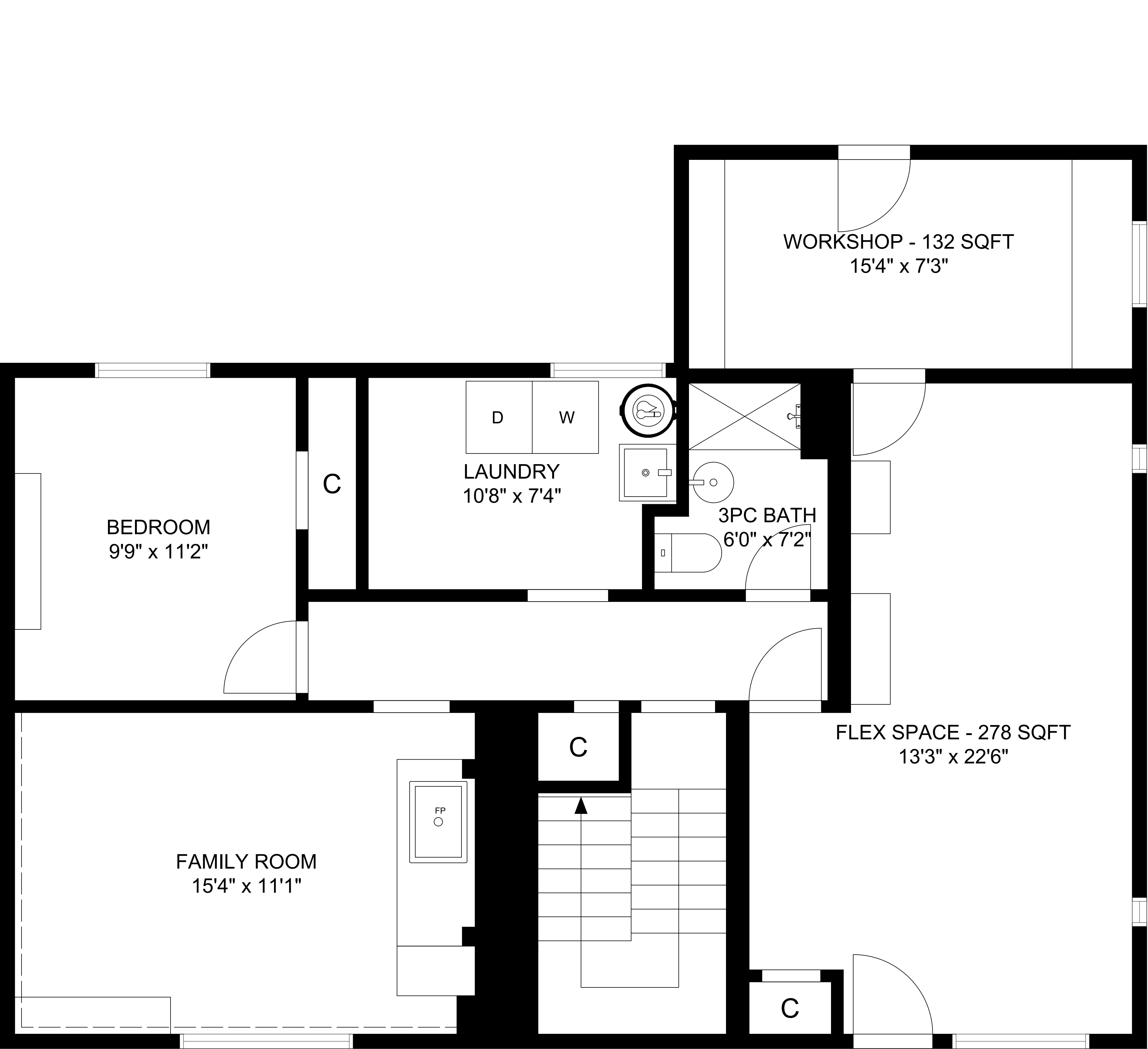
LOWER LEVEL - 656 SQFT CEILING HEIGHT - 6'10"
