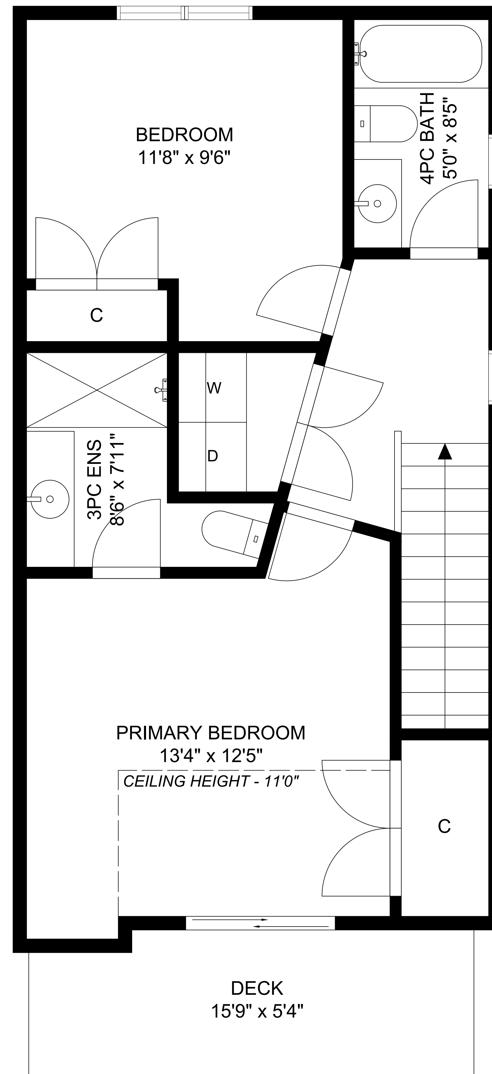
UPPER LEVEL - 616 SQFT CEILING HEIGHT - 8'0"
