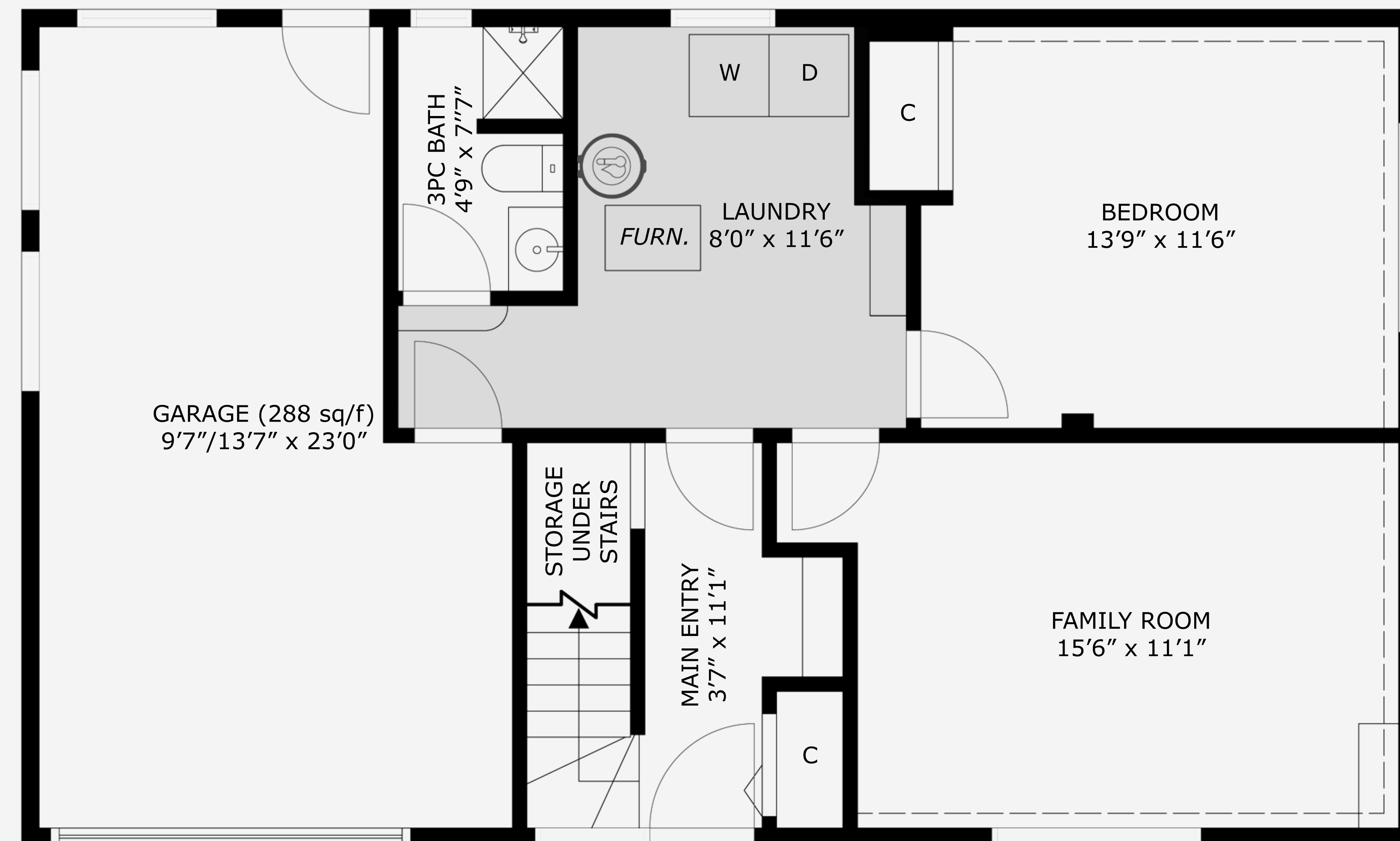
LOWER LEVEL (FINISHED - 542 sq/f, UNFINISHED - 126 sq/f) CEILING HEIGHT - 8'0"
